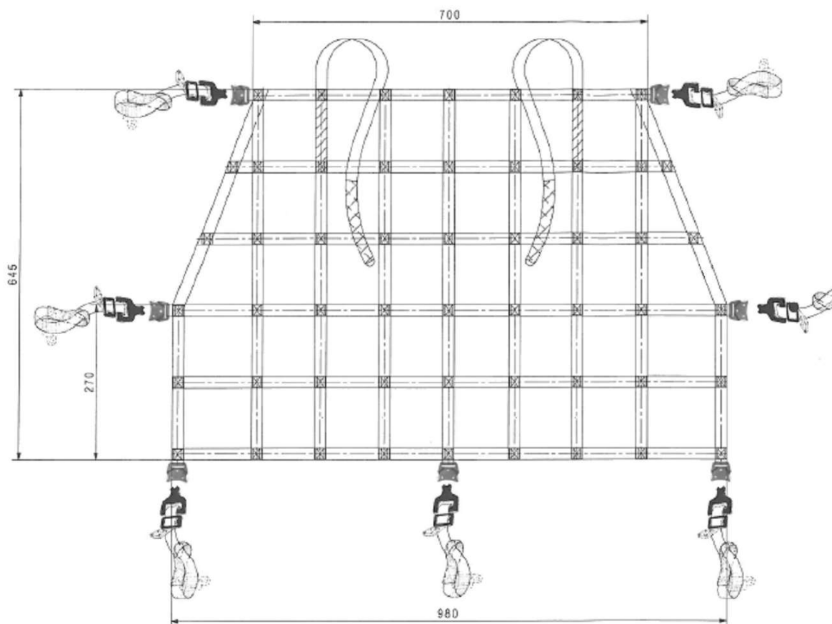
Figure 1 - DA 40 NG baggage net installation.
